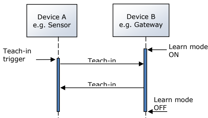
Figure 13. Schematic representation of the teach-in procedure
